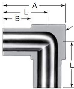
Elbow
